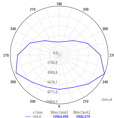
y Cone Curve
