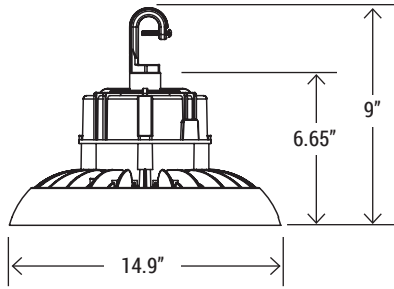
Hook Mount
