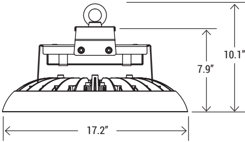
Hook Mount
