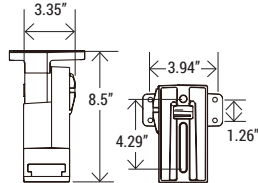
SPM-AL1 / SPM-W-AL1 Adjustable Mount For Square Pole
