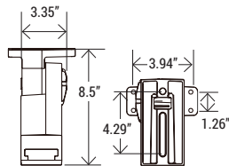
SPM-AL1 / SPM-W-AL1 Adjustable Mount For Square Pole
