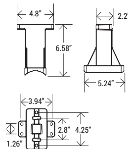
SAM-AL1 / SAM-W-AL1 Straight Arm Mount for Square Pole
