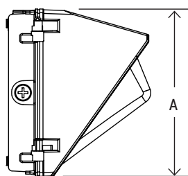
Sid View
