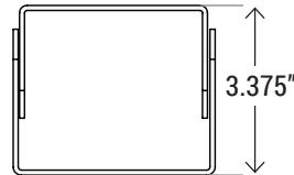
TM-AL2 Trunnion Mount
