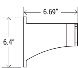
SAM-AL2 Straight Arm Mount for Square Pole
