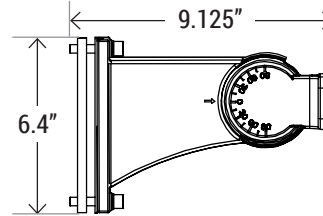
SPM-AL2 Adjustable Mount For Square/Round Pole
